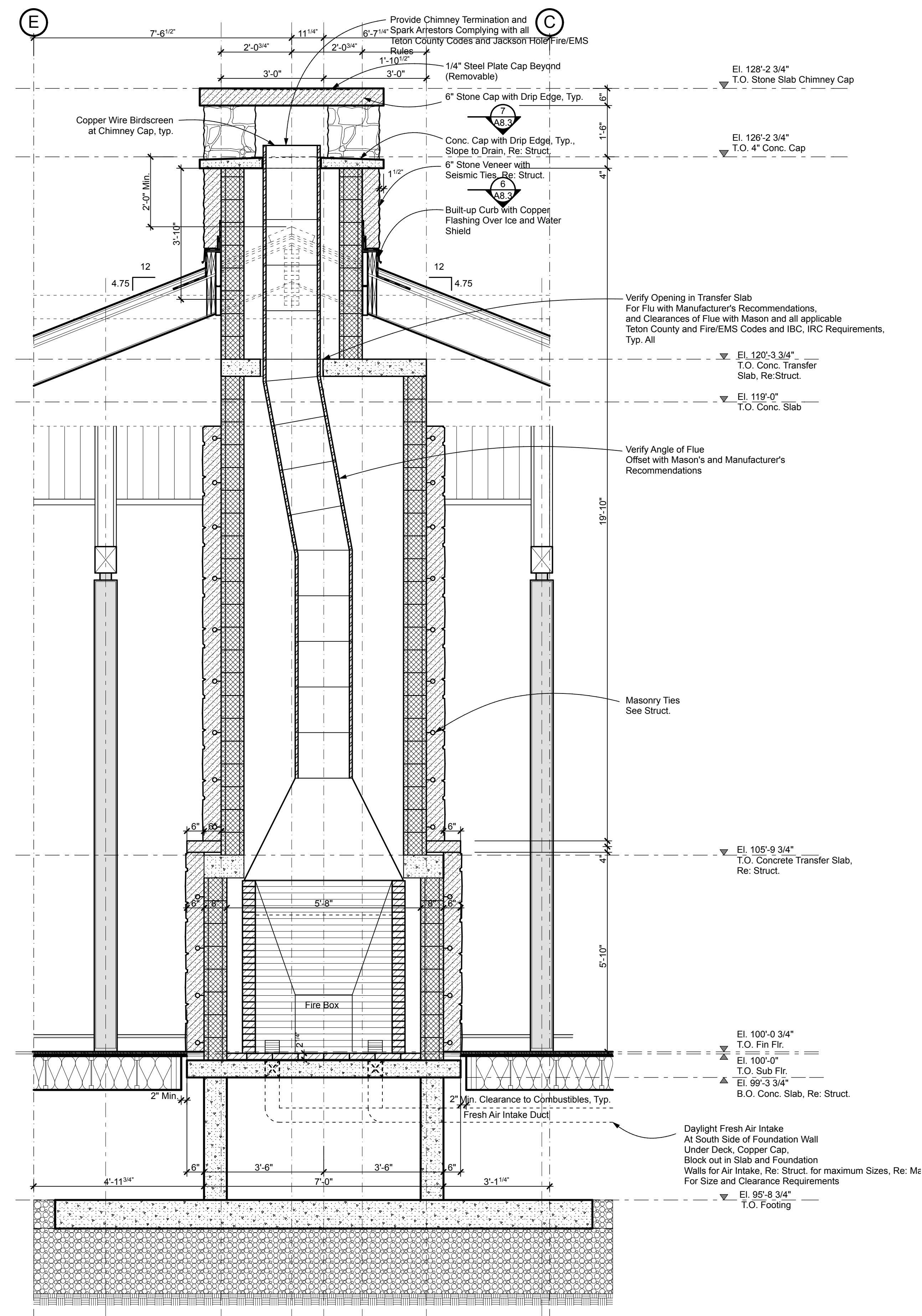
1 Fireplace Section
